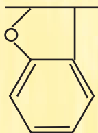
(Coumarone)
